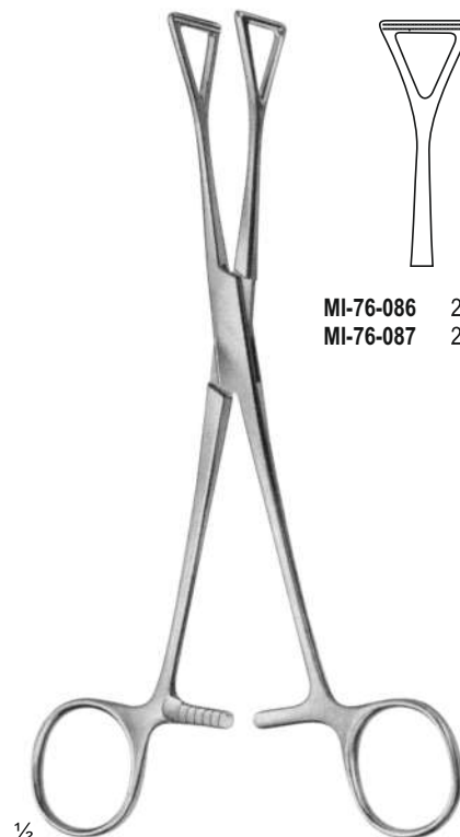
Collin MI-76-087 - MI-76-087 20 cm Intestinal grasping forceps
