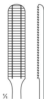
MI-422-062 Drawing cut 34 x 7 mm
