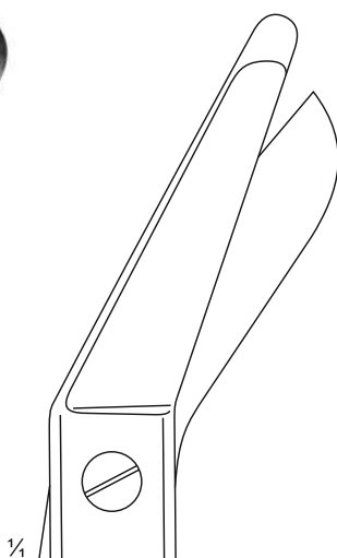
Esmarch MI-228-005 20 cm Plaster shear heavy pattern, short blades
